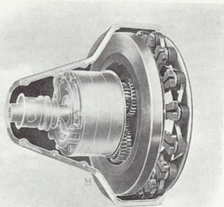
MAGNETO—Showing method of Construction
