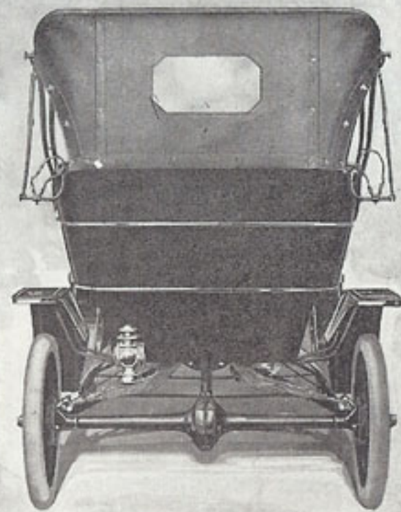
Illustrating Four Posi- tions of the Model T Touring Car with Top
