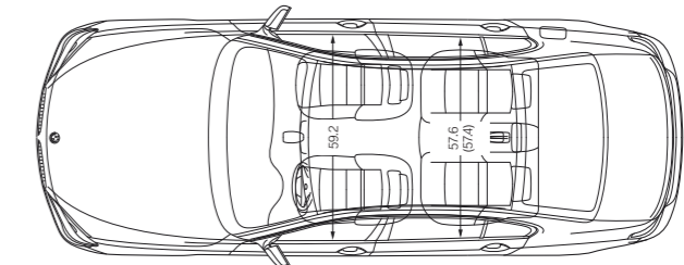
Technical drawing dimensions of 7 Series long-wheelbase models shown in inches. Figures in ( ) refer to the 740i, 750i (short-wheelbase version).
