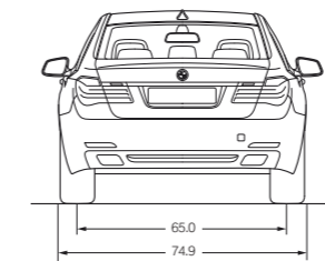
Technical drawing dimensions of 7 Series long-wheelbase models shown in inches. Figures in ( ) refer to the 740i, 750i (short-wheelbase version).
