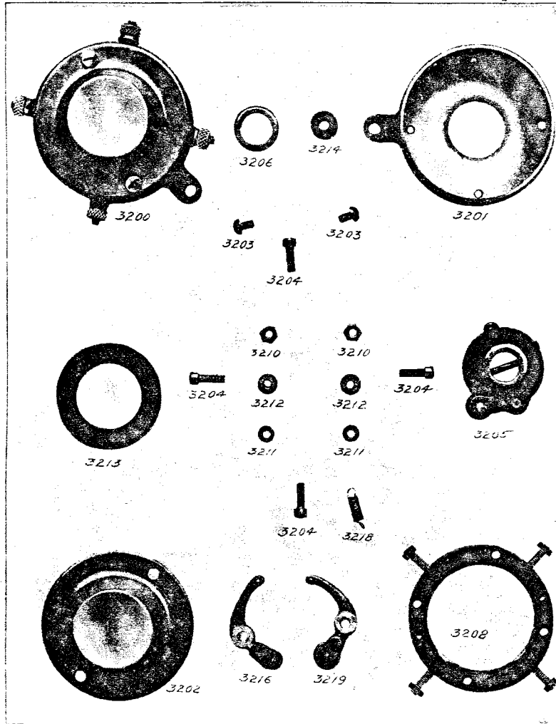
Plate 9—Commutator Parts
