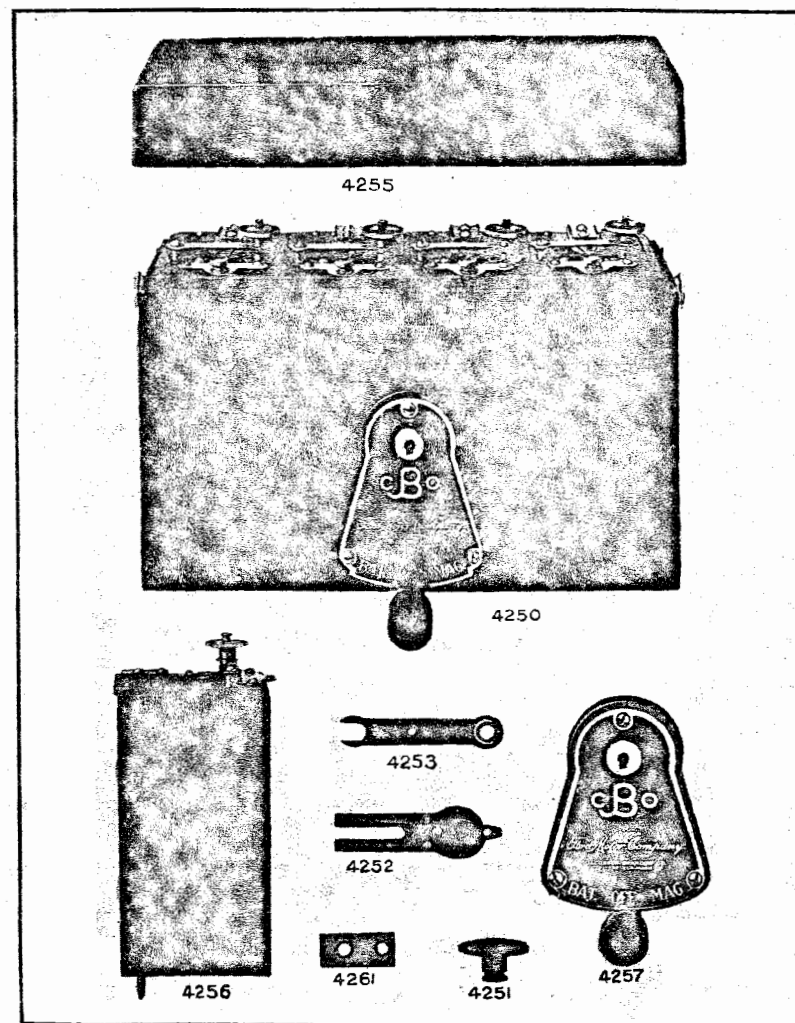
Plate 23—Jacobson-Brandon Coil and Parts
