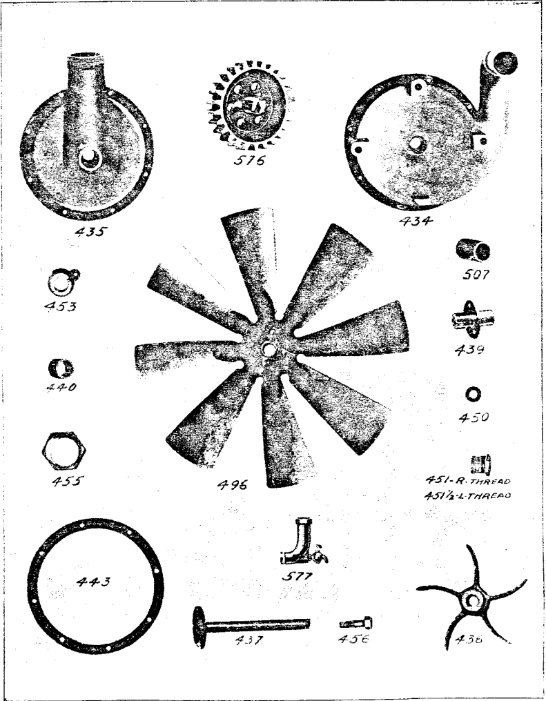
Plate 16—Parts for Pump Circulation Motor
