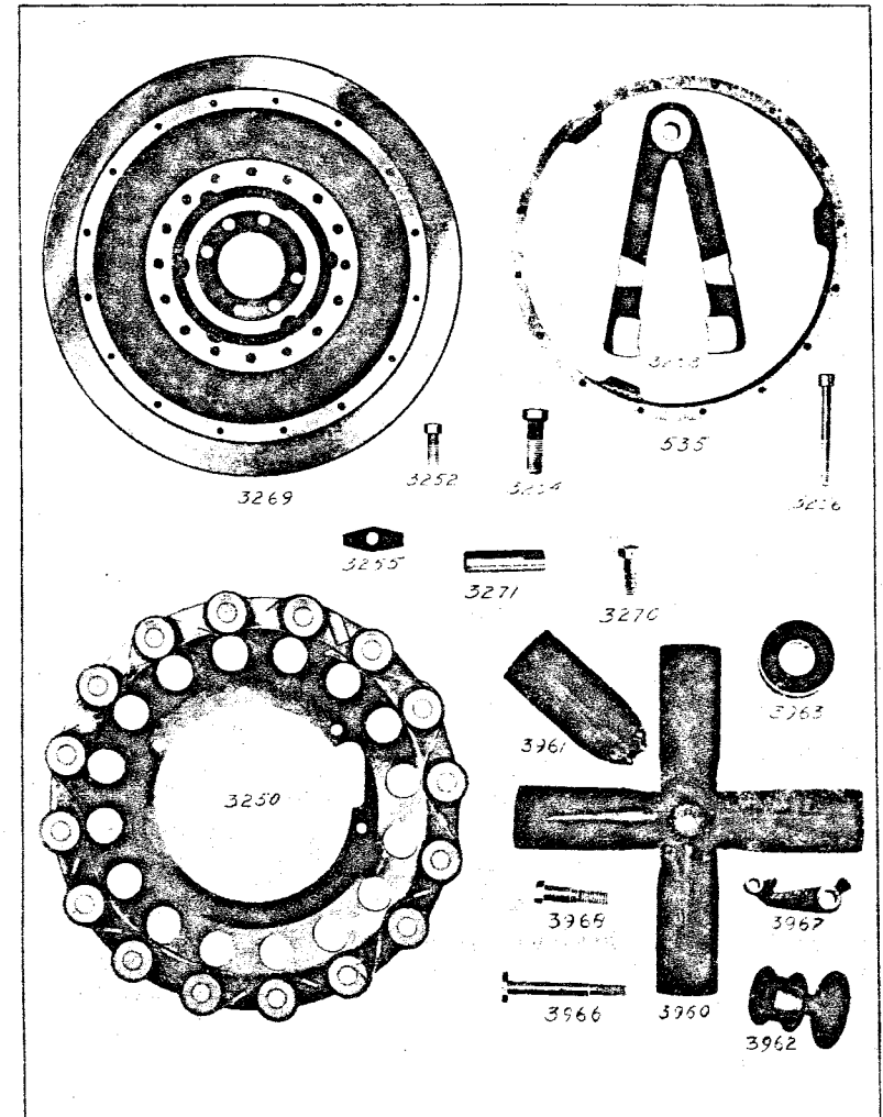
Plate 10—Fly Wheel, Magneto and Fan Parts
