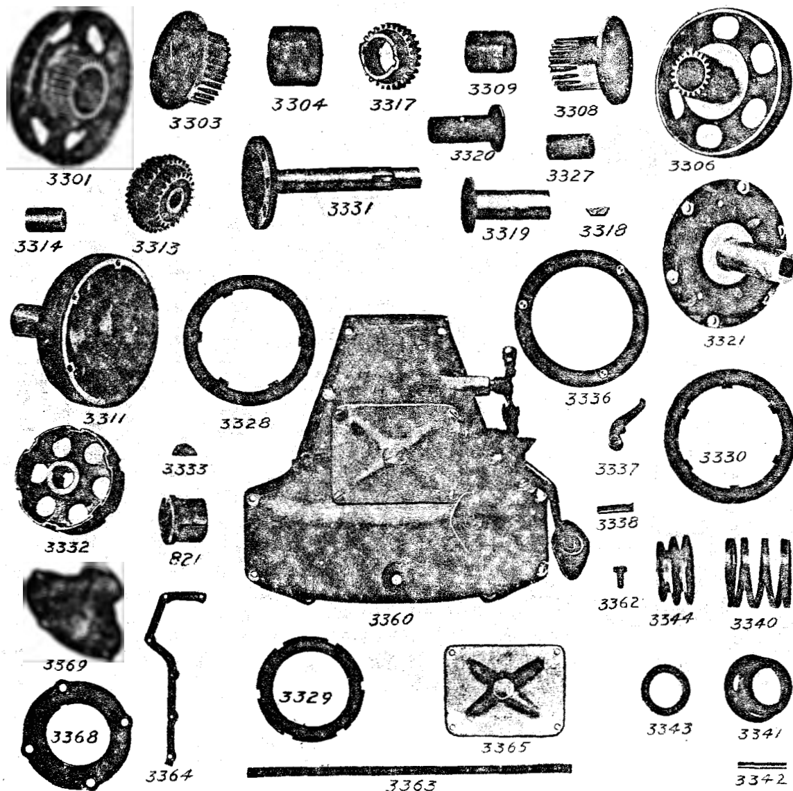
Plate 11—Transmission Parts
