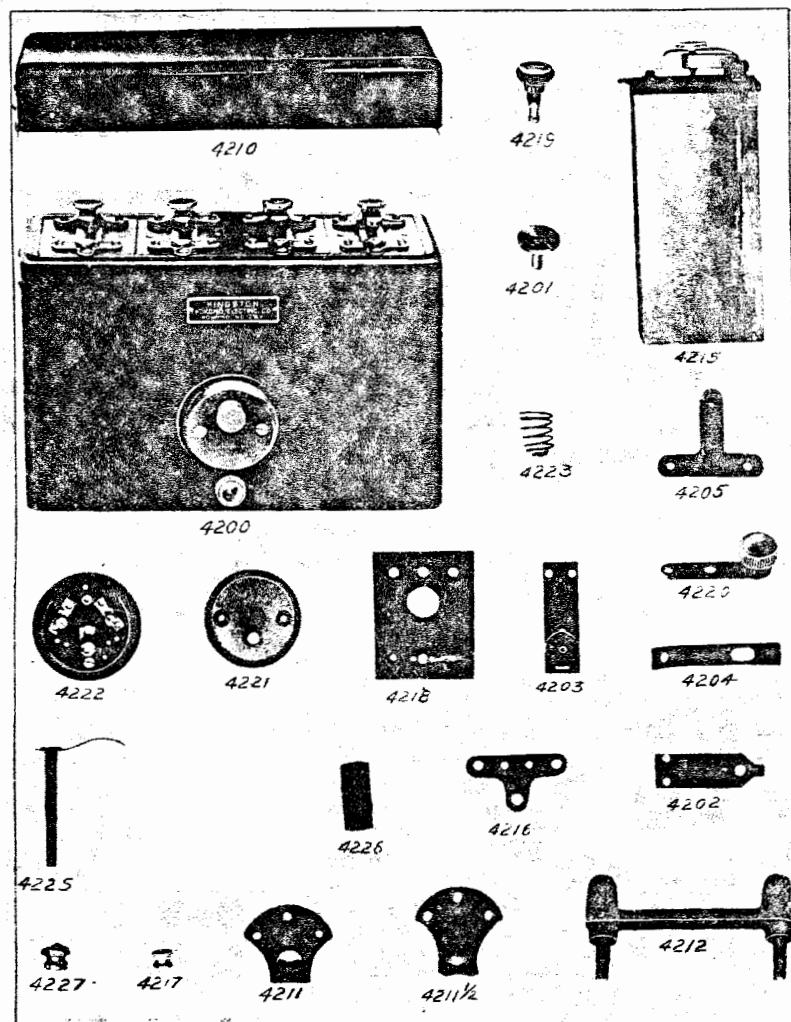
Plate 22—Kingston Coil and Parts
