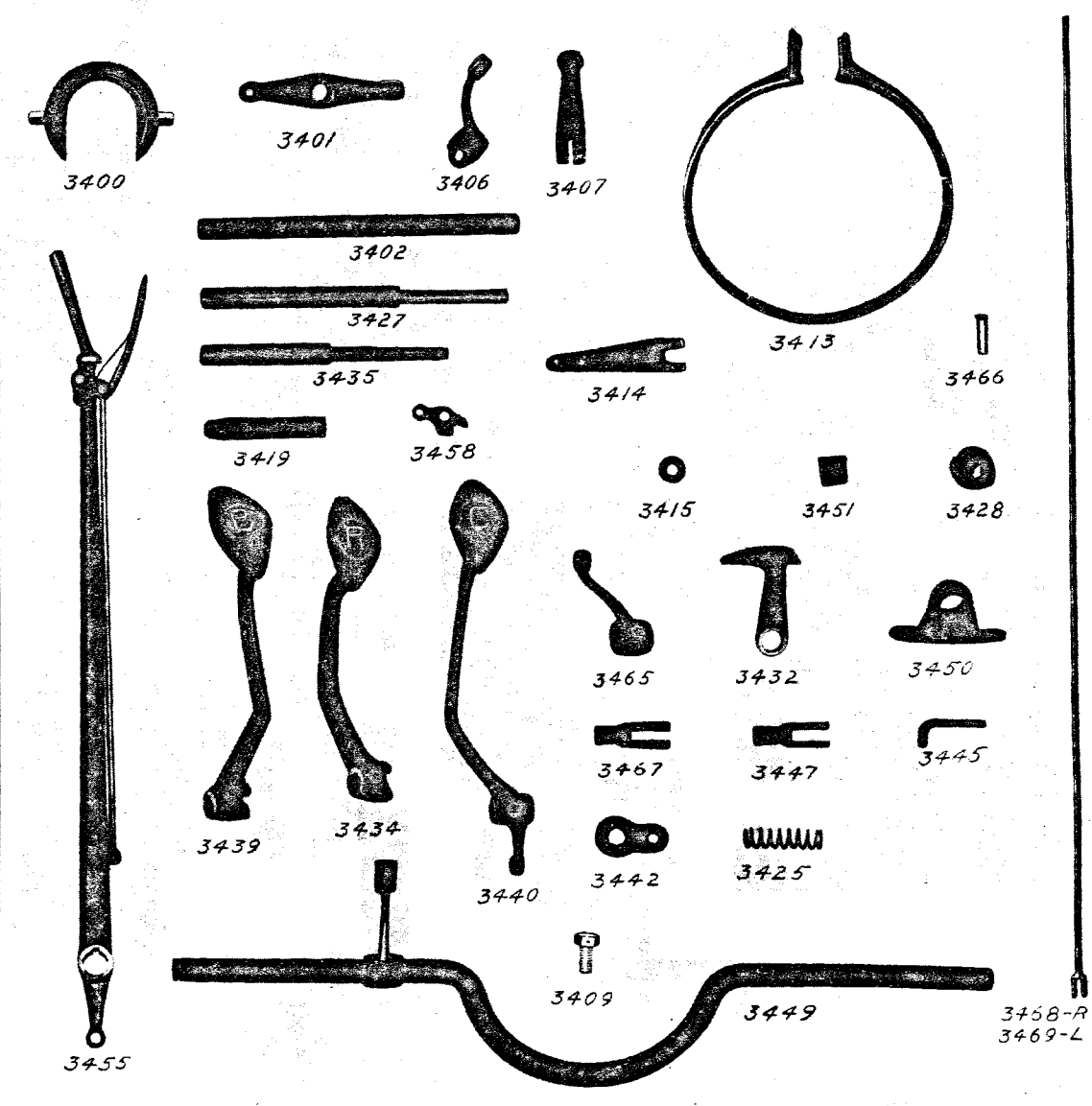
Plate 12—Control Parts
