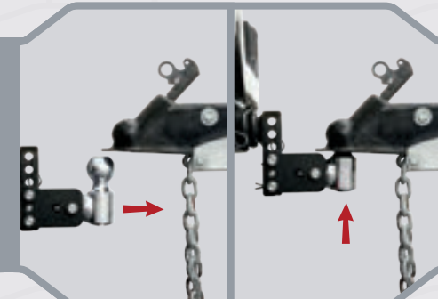
BED-LOWERING MODE WITH AIR SUSPENSION
