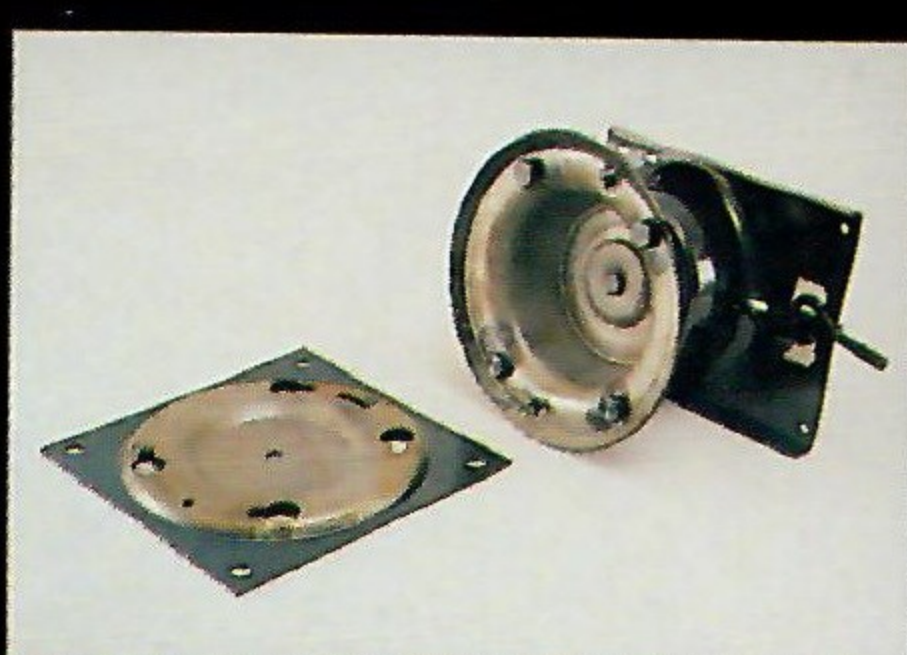
Quick release non-welded stamped steel pedestal
