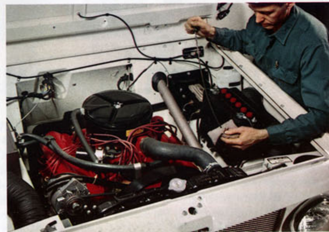
Routine servicing is a snap — All three Scout engines are nestled in a large, low compartment. Distributor, plugs, coil and air filters can be reached without groping. Oil and other routine checks can be made from the front.
