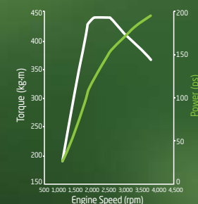
2.2 E-VGT Diesel Engine
