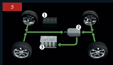
FIG. 5: REGENERATIVE BRAKING
