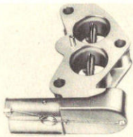
Governor available at extra cost; guards against excessive engine and road speeds.
