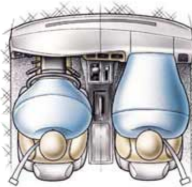
4Runner's Driver and Front Passenger Airbags
