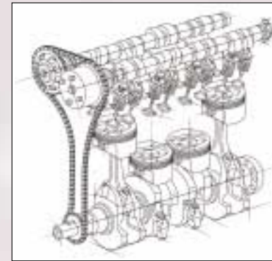
Above: Advanced Variable Valve Timing with intelligence (VVT-i) engine.
