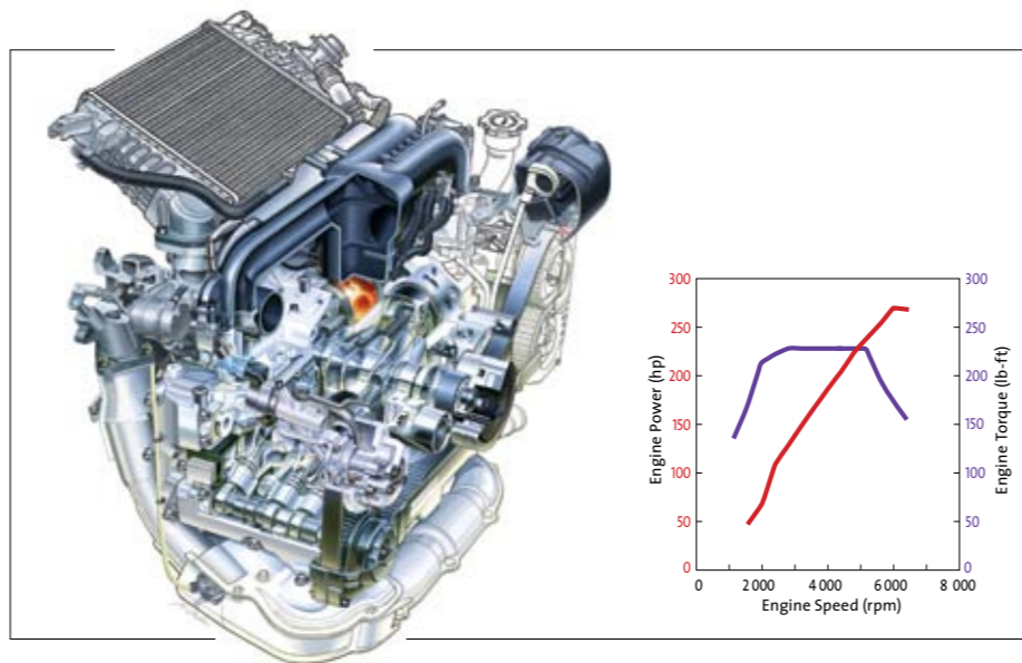
2.5-LITRE DOHC TURBOCHARGED SUBARU BOXER ENGINE HORSEPOWER: 265 HP @ 6000 RPM TORQUE: 244 LB-FT @ 4000 RPM FUEL ECONOMY (L/100 KM): CITY 11.3 / HWY 8.1 (5MT)
