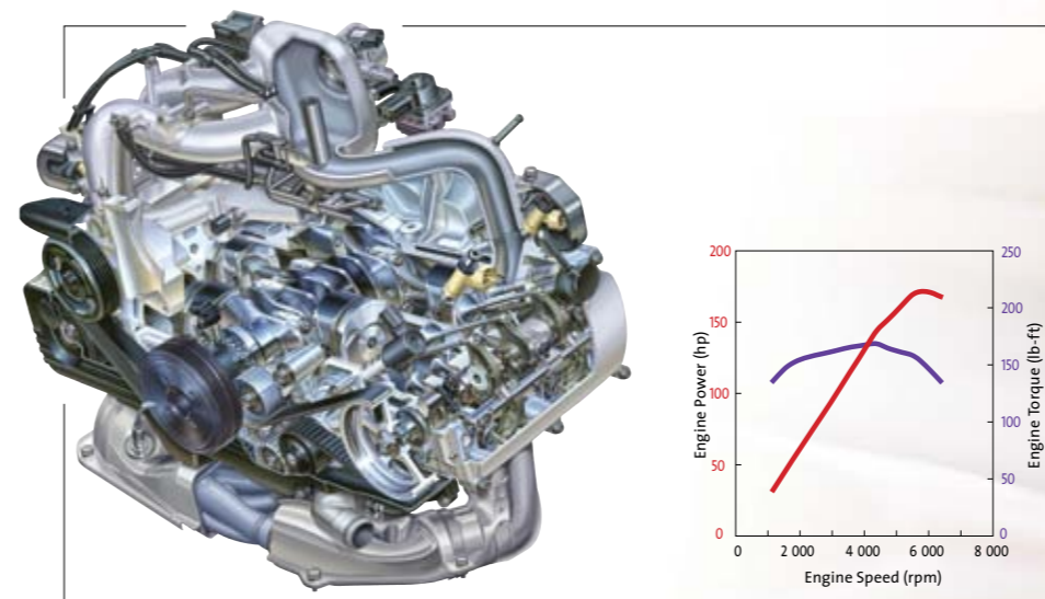
2.5-LITRE SOHC SUBARU BOXER ENGINE HORSEPOWER: 170 HP @ 6000 RPM TORQUE: 170 LB-FT @ 4400 RPM FUEL ECONOMY (L/100 KM): CITY 10.6 / HWY 7.5 (5MT) CITY 10.4 / HWY 7.7 (4EAT 5S)
