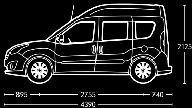
Cargo glazed with standard wheelbase and high roof.
