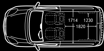
Cargo with standard wheelbase and standard or high roof.
