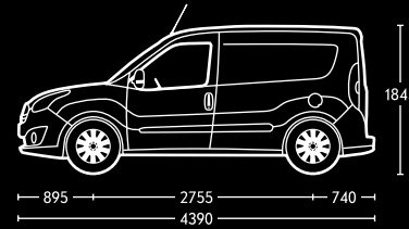
Cargo with standard wheelbase and standard roof.
