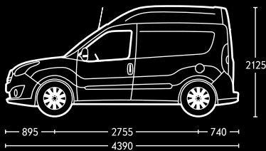
Cargo with standard wheelbase and high roof.
