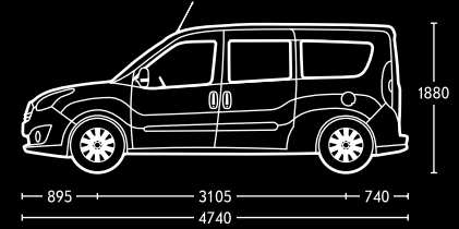
Cargo glazed with long wheelbase and standard roof.
