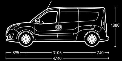
Cargo with long wheelbase and standard roof.
