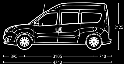
Cargo glazed with long wheelbase and high roof.
