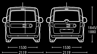
Cargo with asymmetrical rear doors or tailgate.
