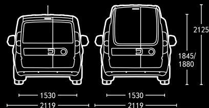
Cargo with standard or high roof.
