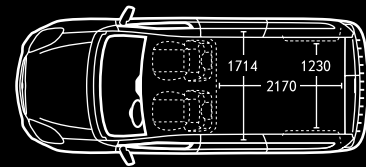
Cargo with long wheelbase and standard or high roof.
