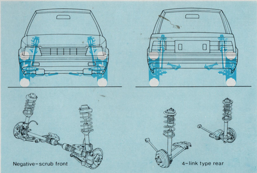
Advanced 4-wheel independent suspension
