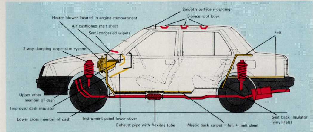
Comprehensive sound insulation
