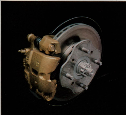
Ventilated front disc brakes
