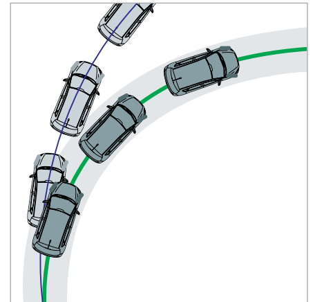
ESP corrects understeering
