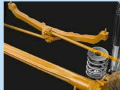
Watt's link improves handling and ride comfort.
