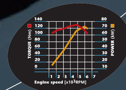
Engine power/torque output 1.4 VVT-i
