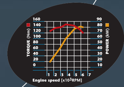
Engine power/torque output 1.6 VVT-i
