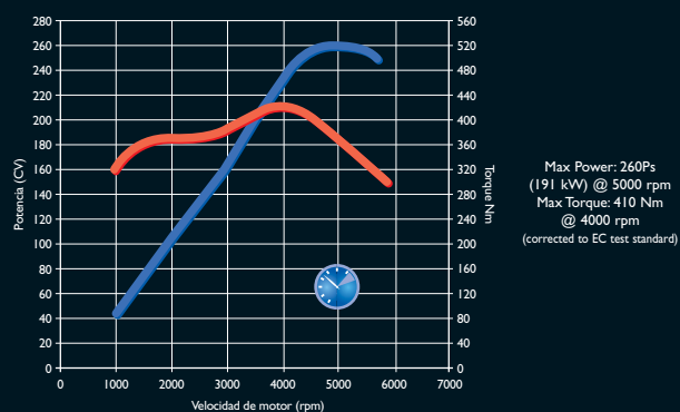
MG ZT 260 POWER CHART
