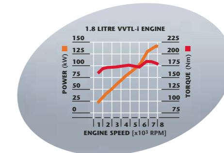
The VVTL-i engine used by the Celica T Sport raises performance to an impressive 141kW of power at 7,800 rpm and 180Nm of torque at 6,800 rpm.
