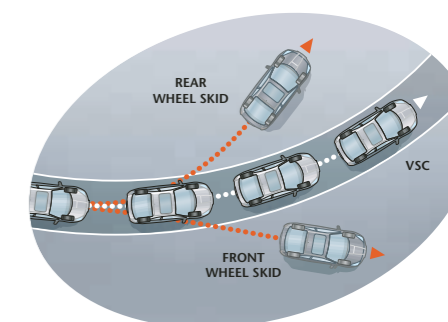
Vehicle Stability Control (VSC), standard on Celica T Sport, aids the driver in controlling sudden understeer and oversteer encountered during cornering.
