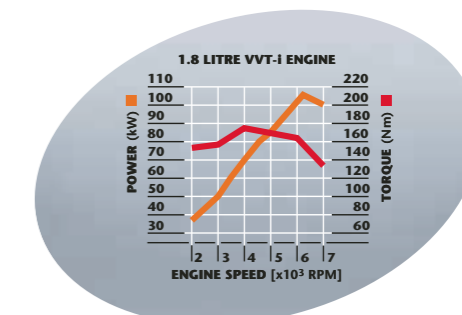
The VVT-i engine develops a maximum 105kW of power at 6,400 rpm with maximum torque of 172 Nm at 4,200 rpm.
