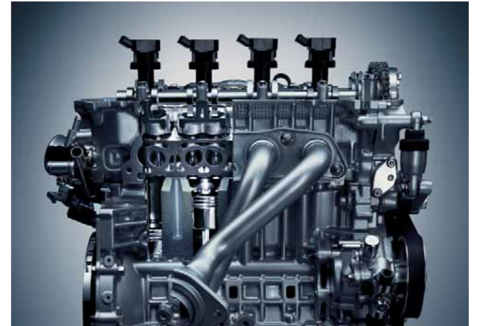
1.8 litre VVT-i engine shown may differ slightly from that in Corolla Verso.
