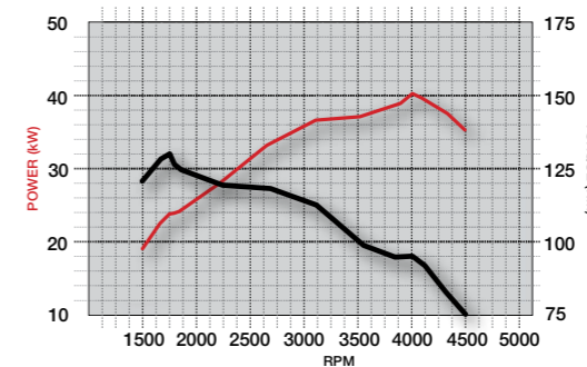
The 1.4-litre diesel engine features high-pressure common-rail diesel technology for quiet yet powerful performance
