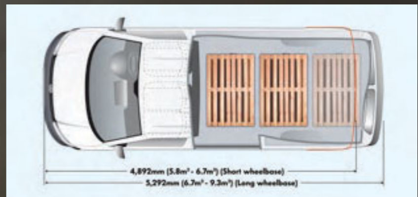
Load floor showing accommodation of euro-pallets.
