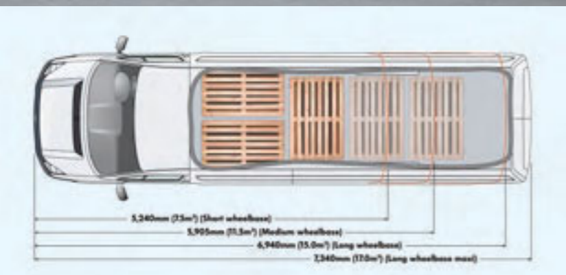
Load floor showing accommodation of euro-pallets.
