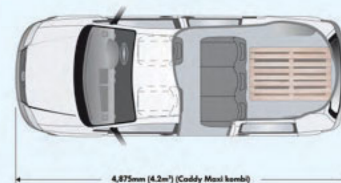
Load floor showing accommodation of euro-pallet.
