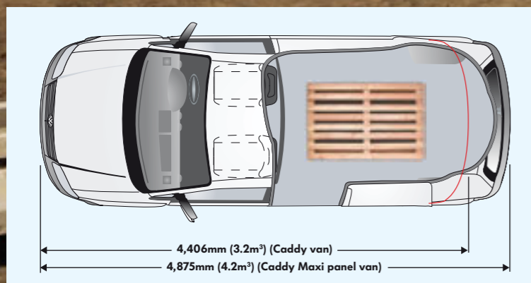
Load floor showing accommodation of euro-pallet.
