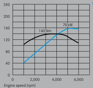
A 160 BlueEFFICIENCY
