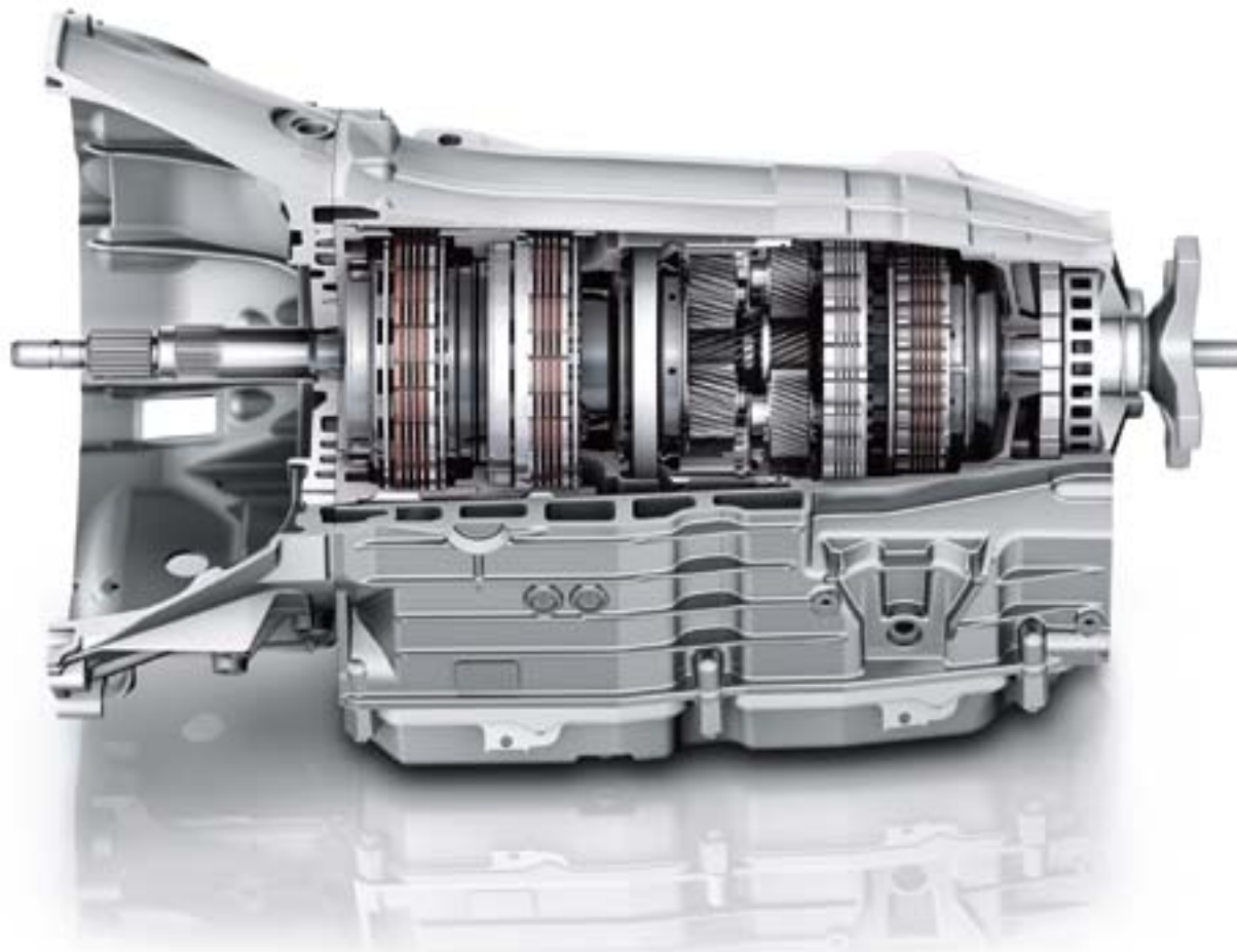
7G-Tronic Plus: the result of more than 50 years' experience in automatic transmission technology
