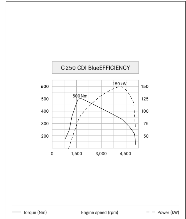
The C 250 CDI BlueEFFICIENCY combines high levels of power and torque with impressive fuel efficiency
