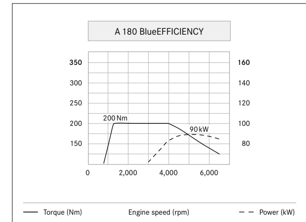
The A 180 BlueEFFICIENCY's new 4-cylinder petrol engine benefits from direct petrol injection, variable valve timing and turbocharging
