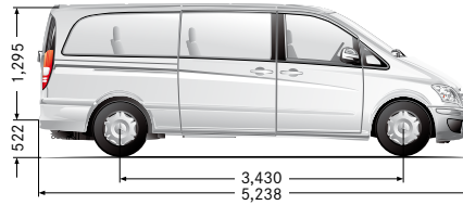
Extra-long version 7
