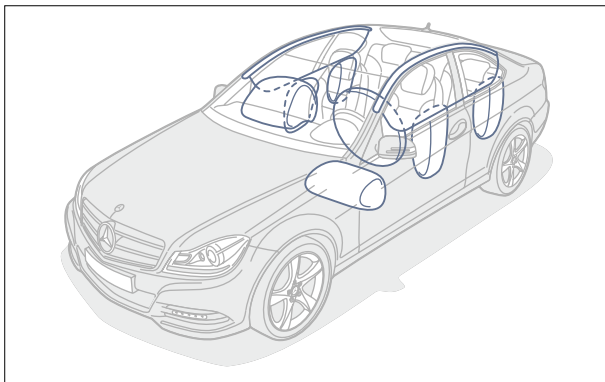
The rigid passenger cell, front and rear crumple zones and intelligent restraint systems provide optimum protection in the event of an impact
