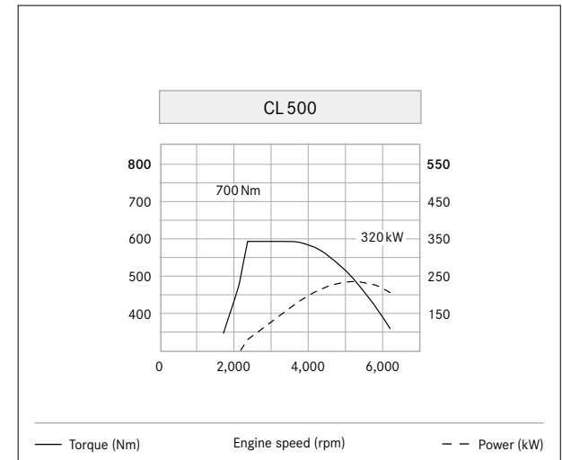
The CL 500: improved power and torque thanks to direct petrol injection and twin turbochargers
