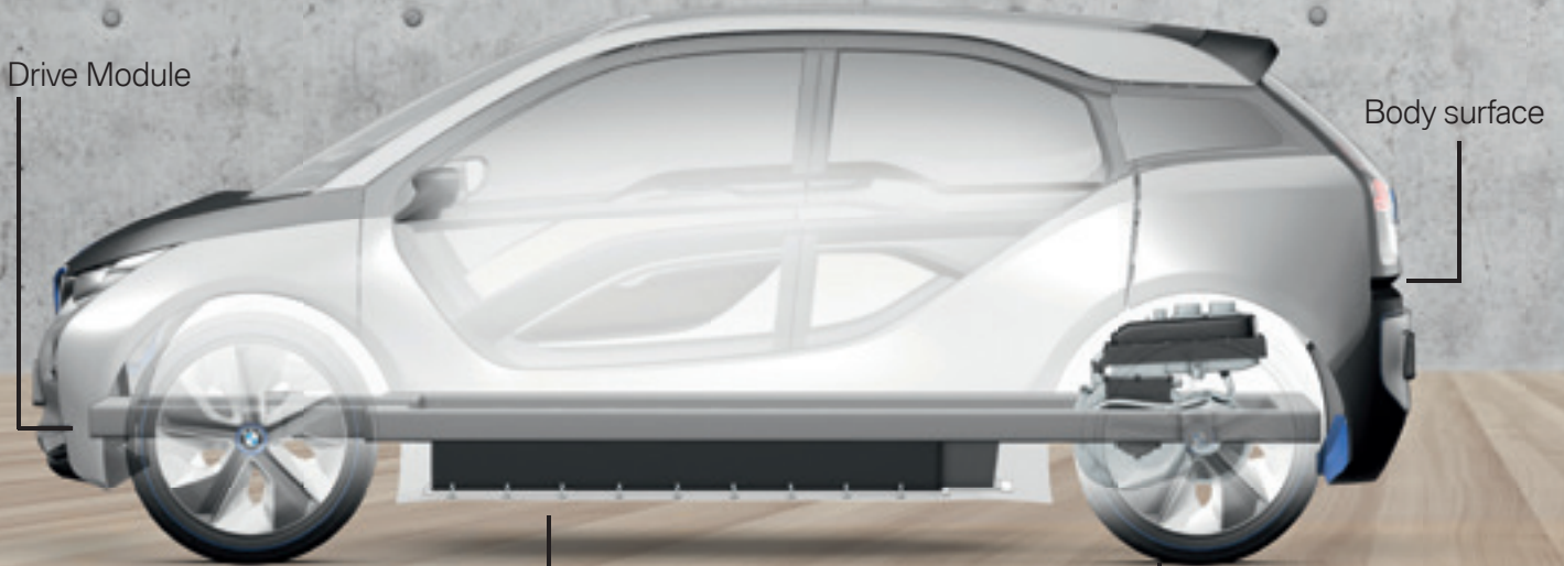
Lithium-Ion Battery
