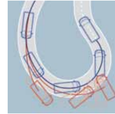
DSC helps avoid understeering and oversteering by correcting the driving line through a combination of brake application to the appropriate wheel and a reduction in engine torque.
