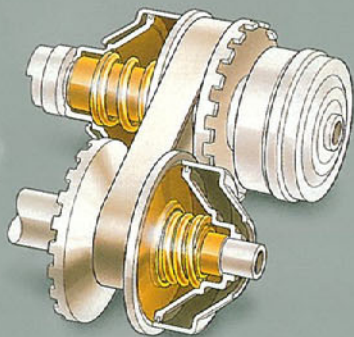
CVT (high transmission ratio).
