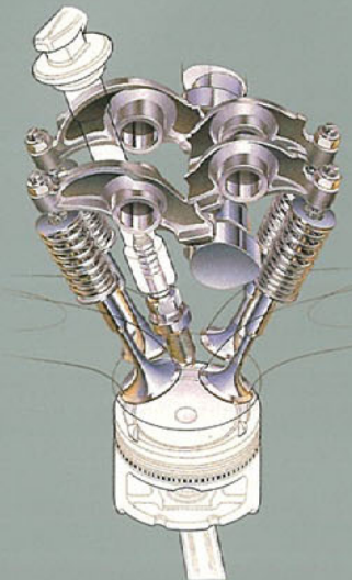
1.6 SOHC 16-valve engine.
