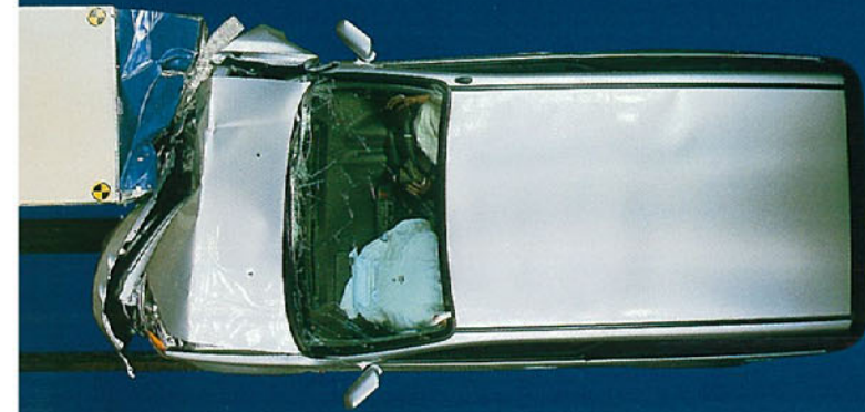
Offset crash test.
