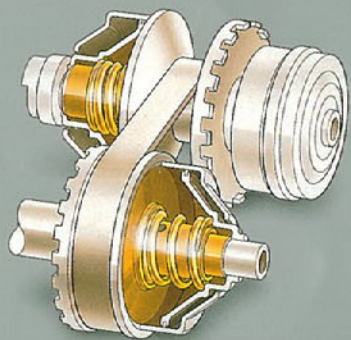
CVT (low transmission ratio).
