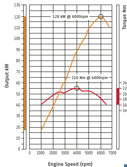
2.4 MIVEC Performance Curves
