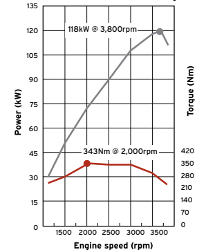
3.2L Common Rail DI-D Engine
