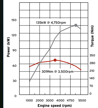
3.5L V6 Engine
