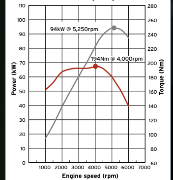
2.4L 4 Cyl Engine
