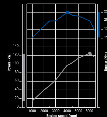
2.4L MIVEC DOHC Engine
