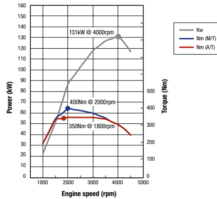
2.5L HP Common Rail DI-D Engine
