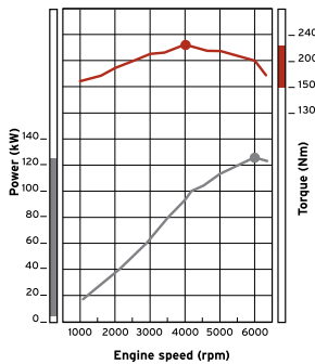
2.4L MIVEC Engine
