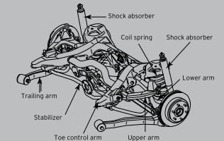
REAR SUSPENSION
