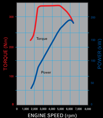
SUBARU WRX 2.5-LITRE, FOUR-CYLINDER DOHC TURBOCHARGED BOXER PETROL ENGINE 1
