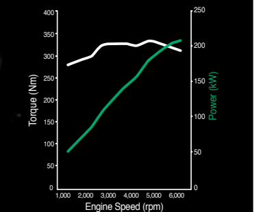
Lambda II 3.5 MPI engine
