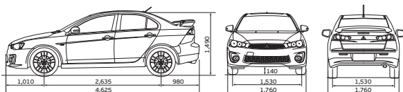
LANCER SEDAN DIMENSIONS (MM)
