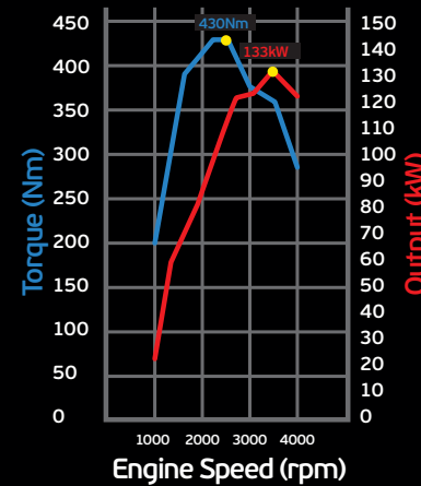
2.4-litre MIVEC turbo diesel engine
