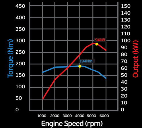
2.4-litre petrol engine
