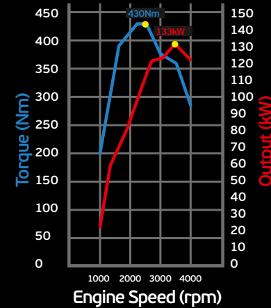
2.4-litre MIVEC turbo diesel engine
