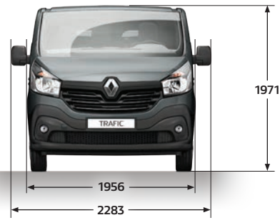
Short Wheelbase
