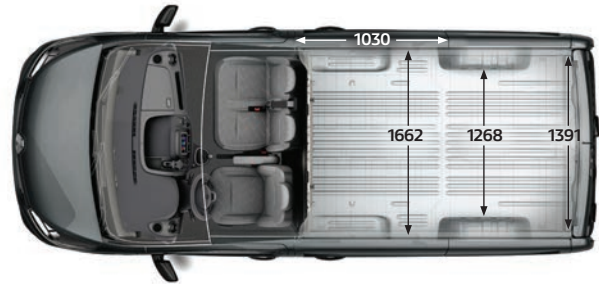
Short Wheelbase
