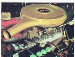
FIERCE PERFORMANCE of 'X2' comes from twin-carburetors, high-performance camshaft, special inlet/exhaust manifolds, plus new exhaust system. Also aluminium alloy main and crank pin bearings.
