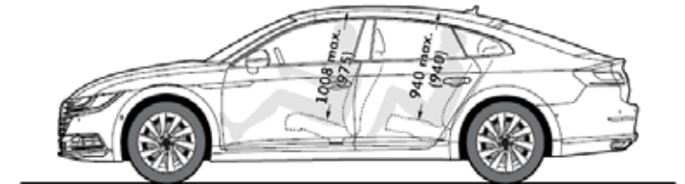
Interior Dimensions#
