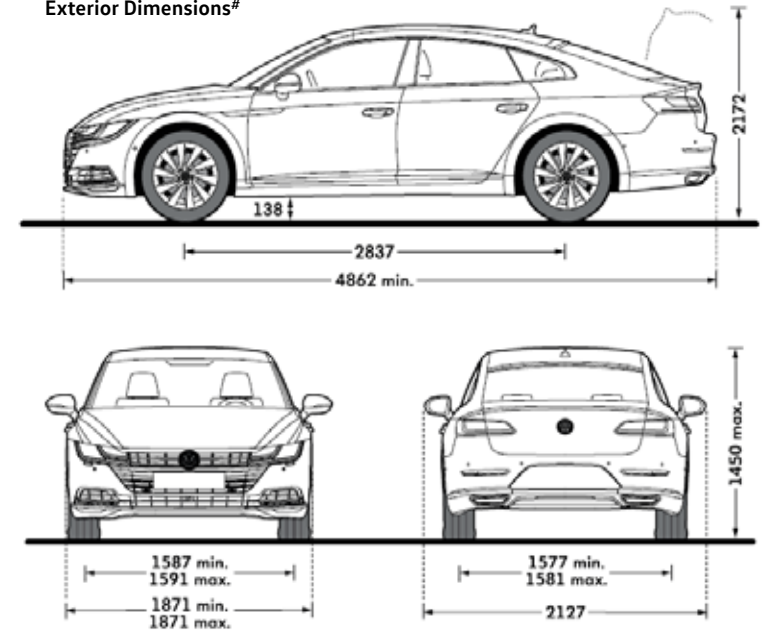
Exterior Dimensions#
