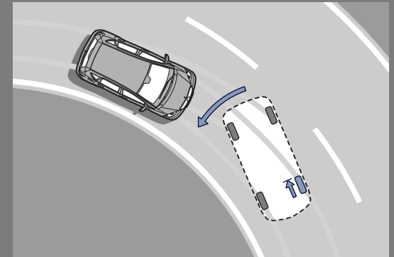
ESP® | Brake application in the event of oversteer
