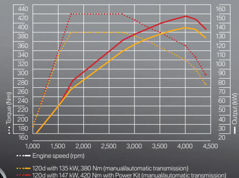
Performance data for the BMW 120d with BMW M Performance Power Kit Full load 120d
