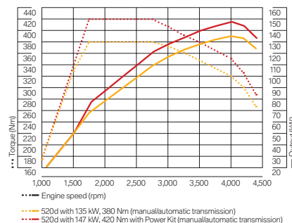
5 Performance data for the BMW 520d with BMW M Performance Power Kit Full load 520d
