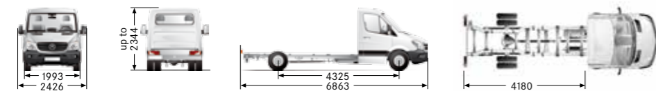
4.49t/5.0t LWB Single Cab Chassis
