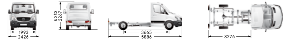
3.55t MWB Single Cab Chassis
