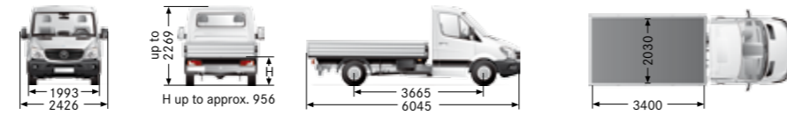
3.55t MWB Single Cab Chassis with tray
