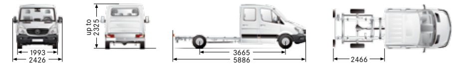
3.55t MWB Dual Cab Chassis
