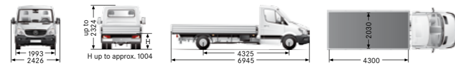
4.49t/5.0t LWB Single Cab Chassis with tray
