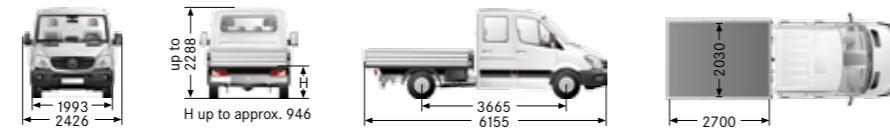
3.55t MWB Dual Cab Chassis with tray
