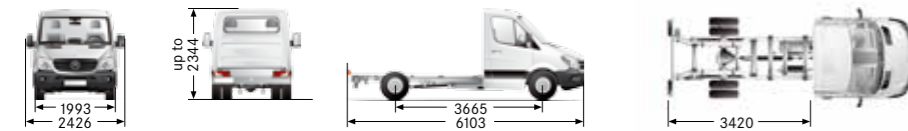
4.49t/5.0t MWB Single Cab Chassis
