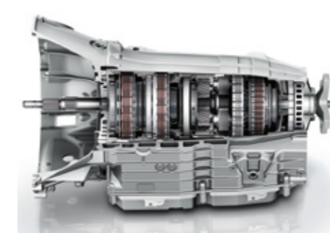
The 7G-TRONIC PLUS automatic transmission offers outstandingly smooth gear changes and potential for saving fuel.
