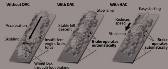
Downhill Assist Control 4,5 and Hill-start Assist Control 4
